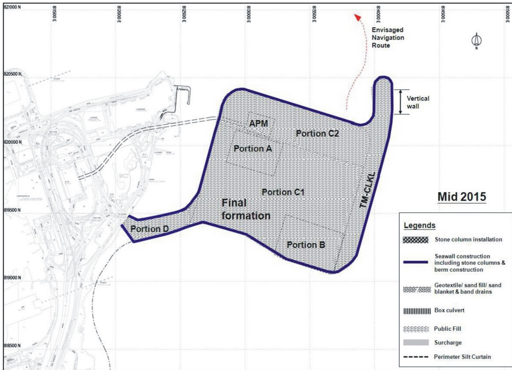
Figure 21 - Outline of Construction Sequence (Sheet 10 of 10)
